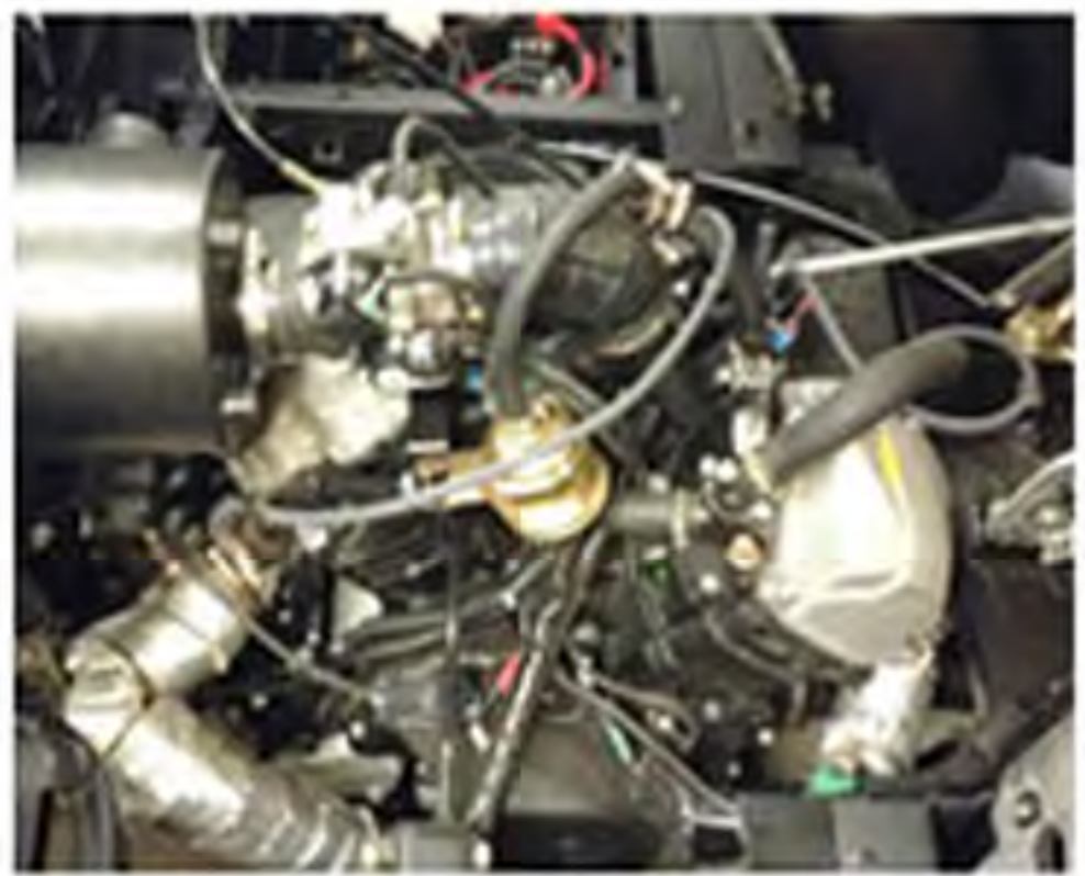
INSULATED HEADERS
